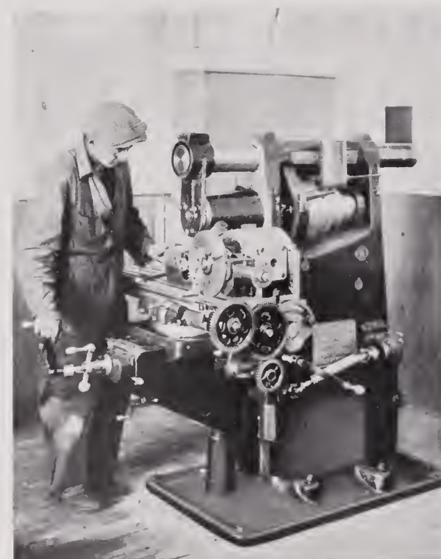
CINCINNATI No. 2 UNIVERSAL MILLER
